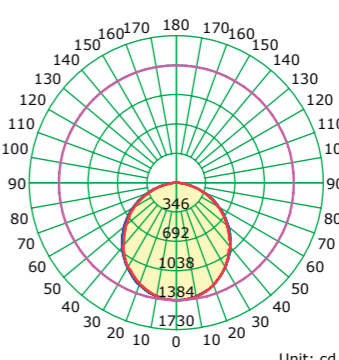
Average Diffuse Angle(50%): 109.4° — C0-C180 — C90-C270 — G1
