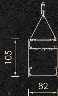
NOTUS 14 LINEAR LED STONE
